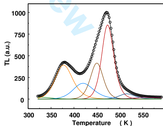
Figure 5 Glow curve of NaF:Eu resolved into individual glow peaks by a computerized glow curve deconvolution (CGCD) analysis.
