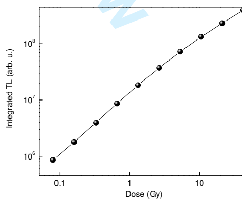
Figure 2 Integrated thermoluminescence as a function of dose, of NaF:Eu 3+ pellets, exposed to \beta particle irradiation in the 0.08 – 42.0 Gy dose range.
