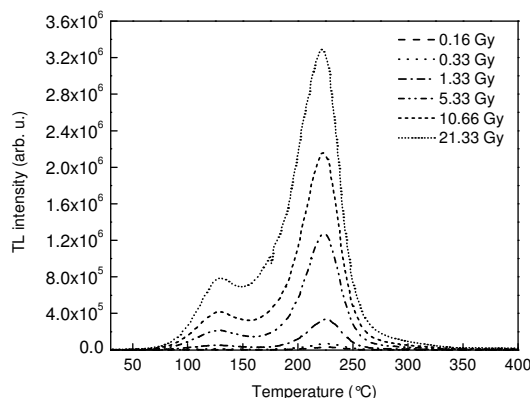
Figure 1 Thermoluminescence glow curves of pellet-shaped sintered NaF:Eu 3+ samples after being exposed to \beta particle irradiation in the dose range from 0.16 to 21.33 Gy.
