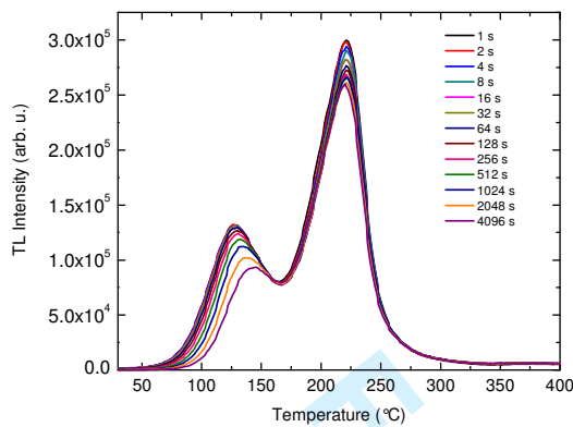
Figure 3 Thermoluminescence glow curves of 2.6 Gy beta irradiated NaF:Eu 3+ , obtained after different elapsed time intervals between irradiation and the corresponding thermoluminescence readout.
