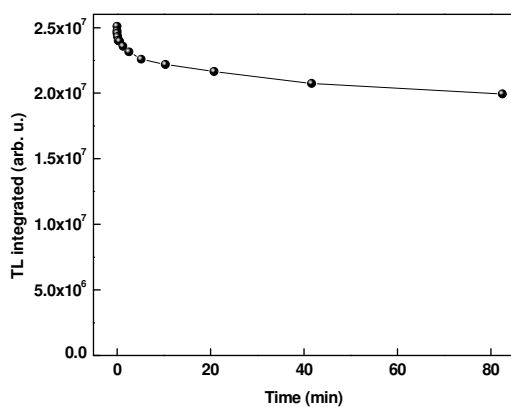
Figure 4 Integrated TL as a function of the time interval elapsed between the irradiation and the corresponding TL readout.
